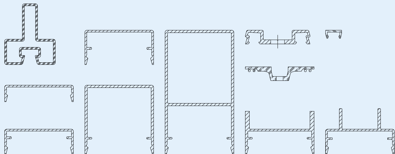
Light effects on the facade through facade cover profiles
