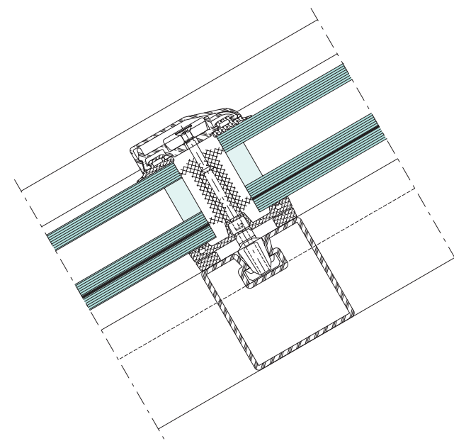
Section detail
