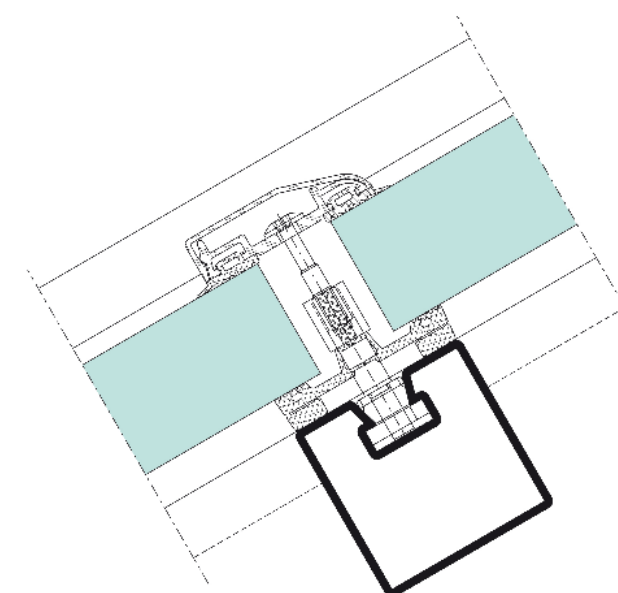
Section detail
