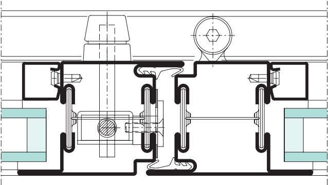
Section detail
