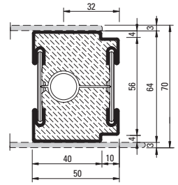
600.010.C4 Z
